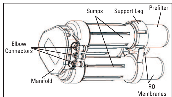
Figure 2 RO Assembly
